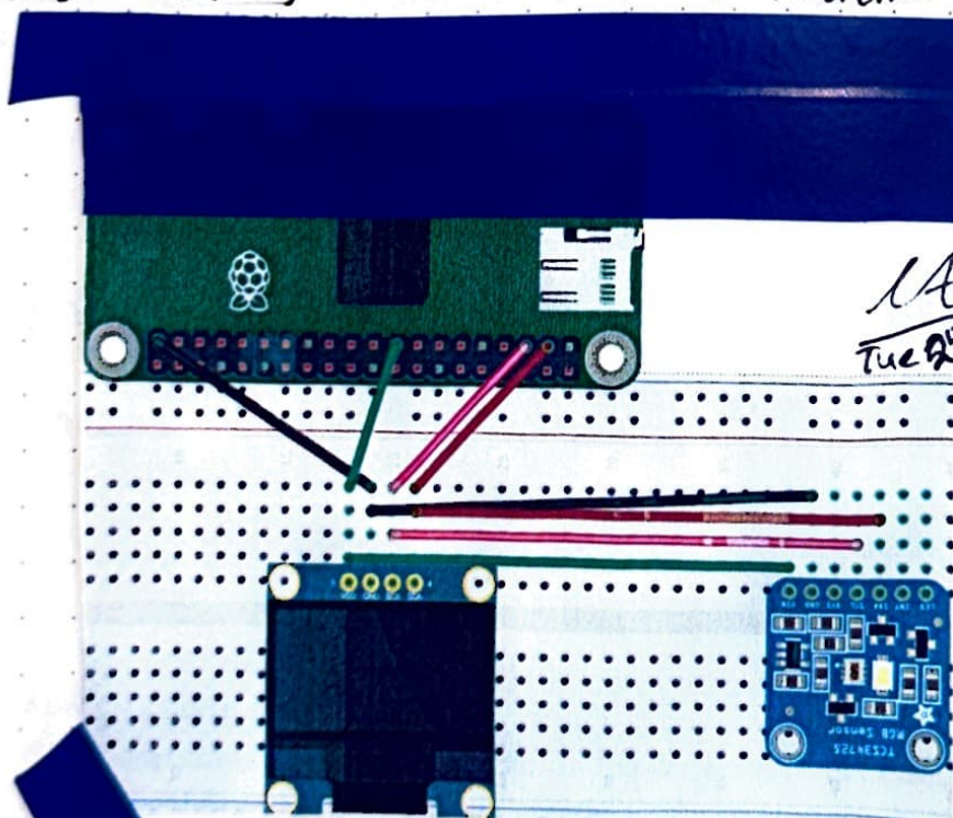
Figure 1: Breadboard wiring, TCS 34725 + SSD1306 Fixing LO.6
